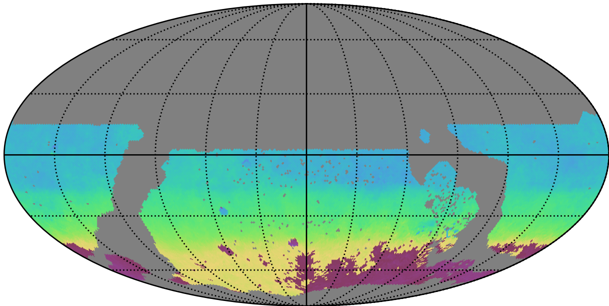
ddf_loaded_fl8_v3.4_10yrs WFD z band: AngleMean rotSkyPos
