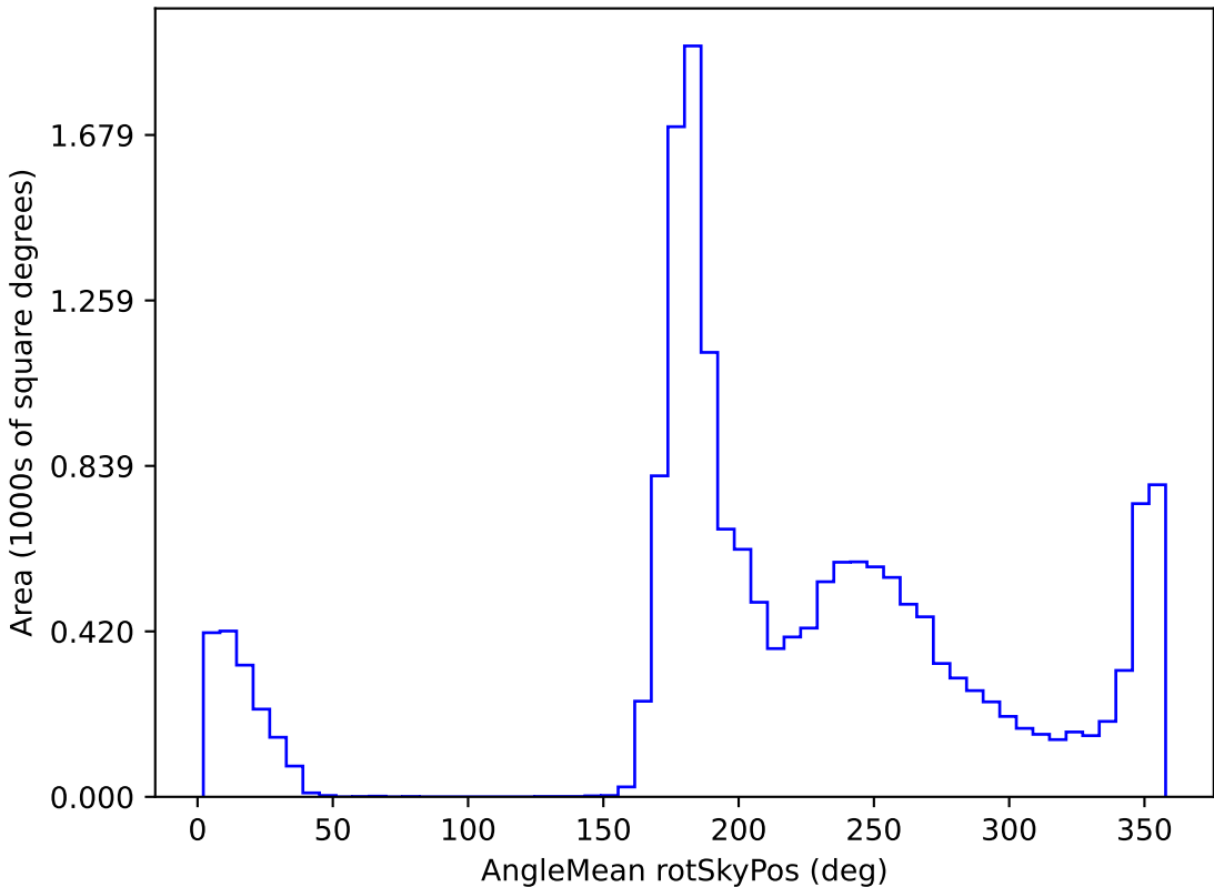
ddf_loaded_fl8_v3.4_10yrs WFD z band: AngleMean rotSkyPos
