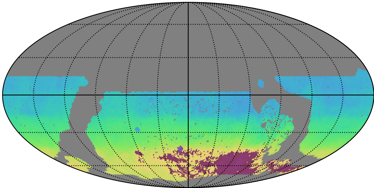
ddf_loaded_fl8_v3.4_10yrs WFD y band: AngleMean rotSkyPos
