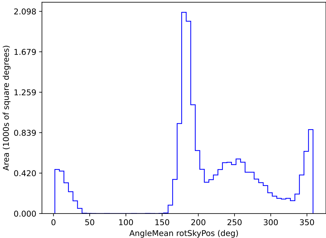
ddf_loaded_fl8_v3.4_10yrs WFD i band: AngleMean rotSkyPos
