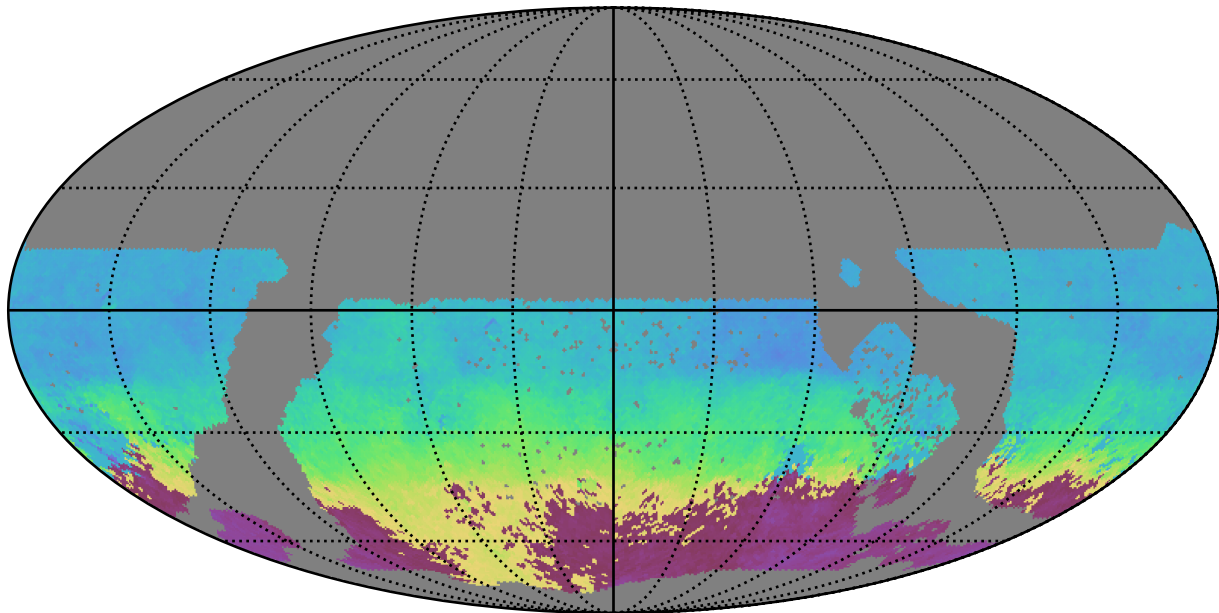
ddf_loaded_fl8_v3.4_10yrs WFD g band: AngleMean rotSkyPos
