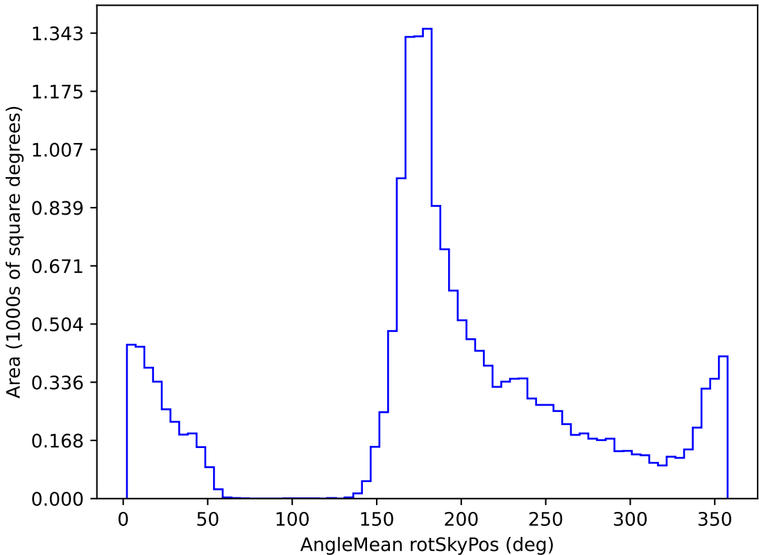
ddf_loaded_fl8_v3.4_10yrs WFD g band: AngleMean rotSkyPos
