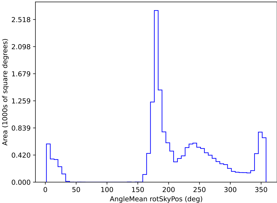
ddf_loaded_fl8_v3.4_10yrs WFD all bands: AngleMean rotSkyPos
