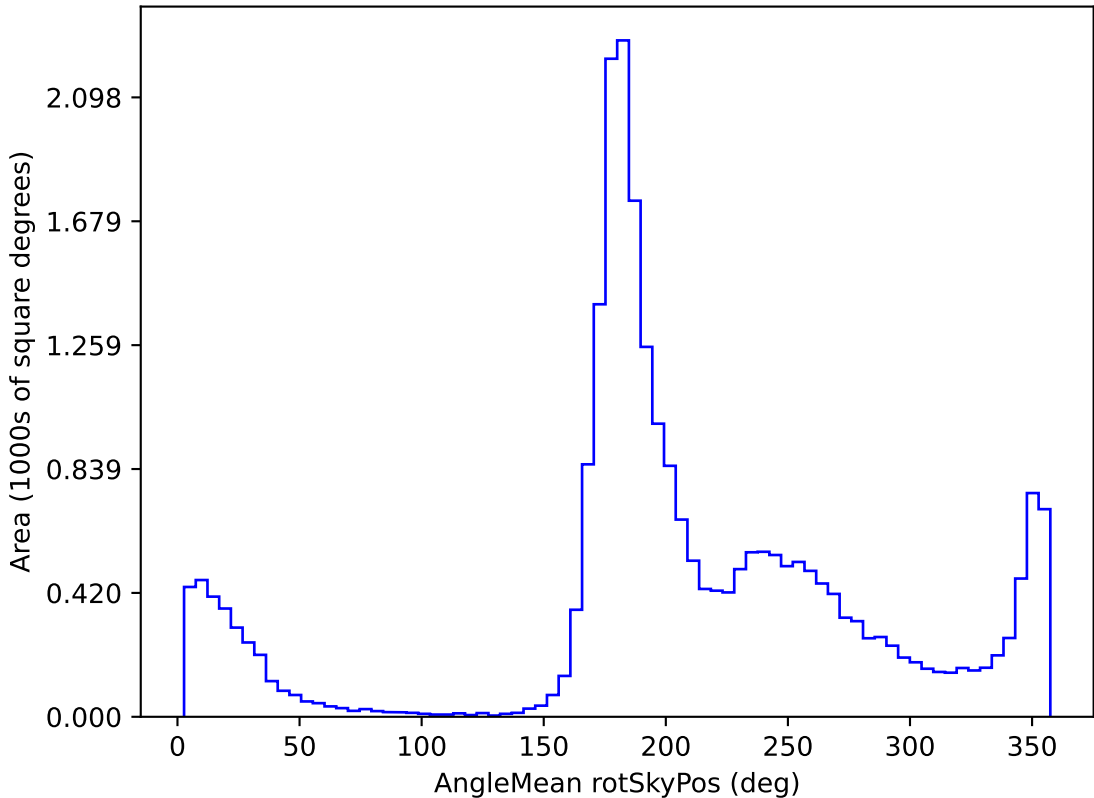
ddf_loaded_fl8_v3.4_10yrs All sky z band: AngleMean rotSkyPos
