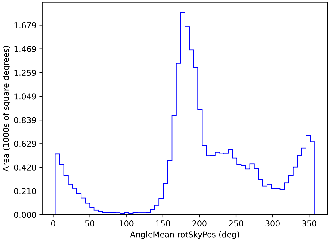
ddf_loaded_fl8_v3.4_10yrs All sky u band: AngleMean rotSkyPos
