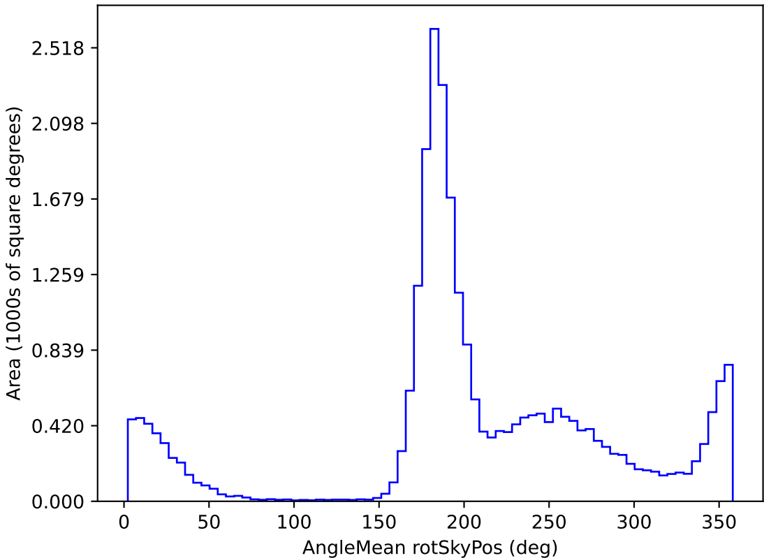
ddf_loaded_fl8_v3.4_10yrs All sky i band: AngleMean rotSkyPos
