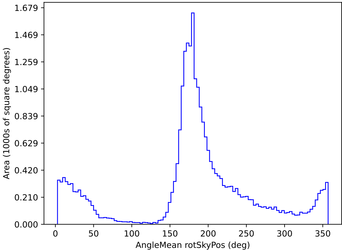
ddf_loaded_fl8_v3.4_10yrs All sky g band: AngleMean rotSkyPos
