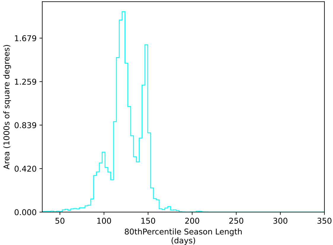
ddf_loaded_fl8_v3.4_10yrs WFD u band: 80thPercentile Season Length
