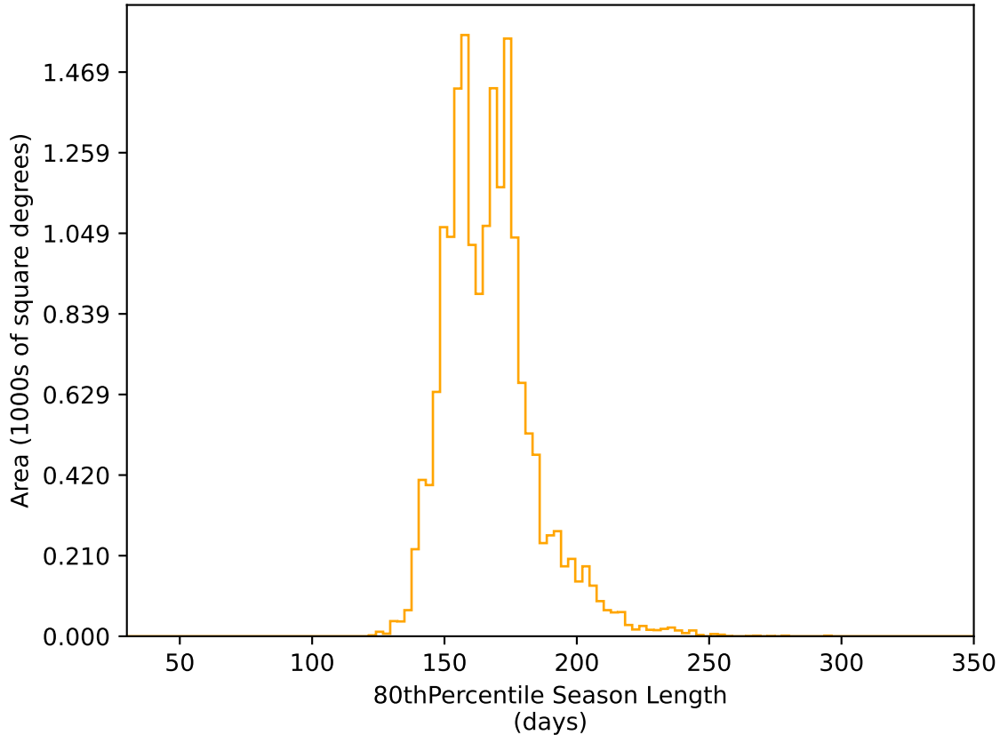
ddf_loaded_fl8_v3.4_10yrs WFD r band: 80thPercentile Season Length
