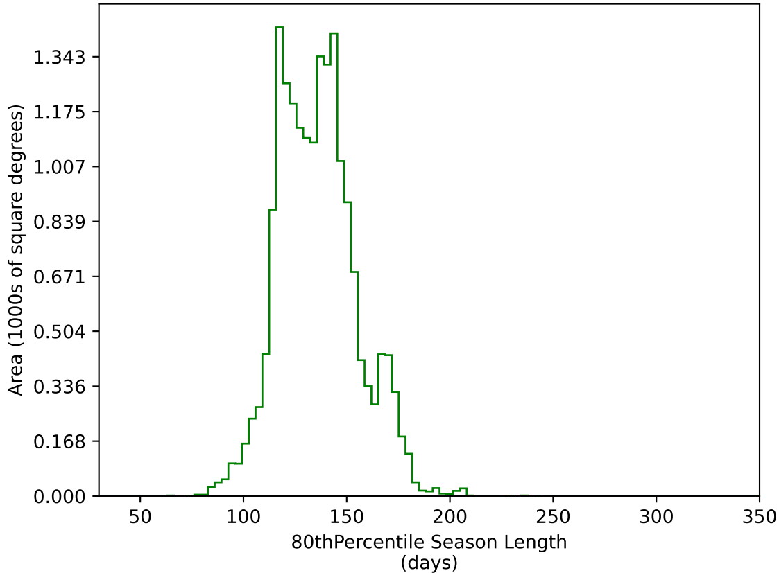
ddf_loaded_fl8_v3.4_10yrs WFD g band: 80thPercentile Season Length
