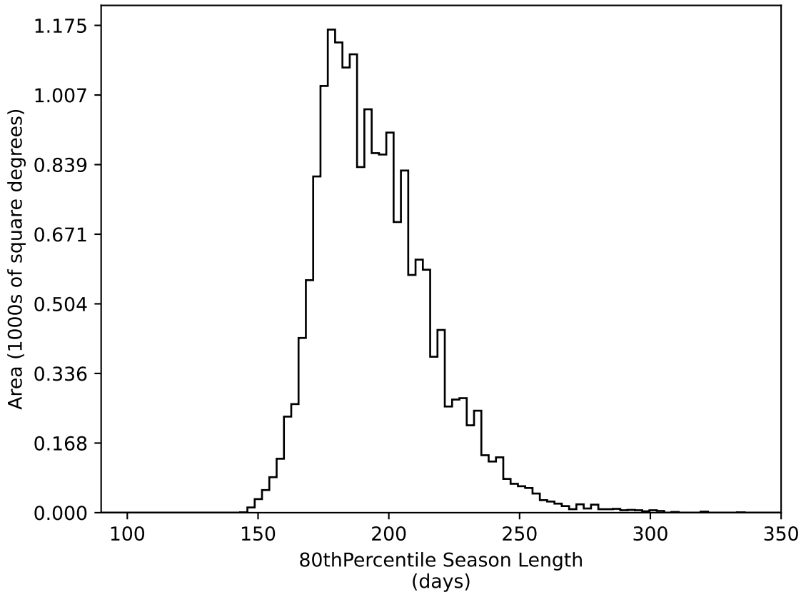
ddf_loaded_fl8_v3.4_10yrs WFD all bands: 80thPercentile Season Length
