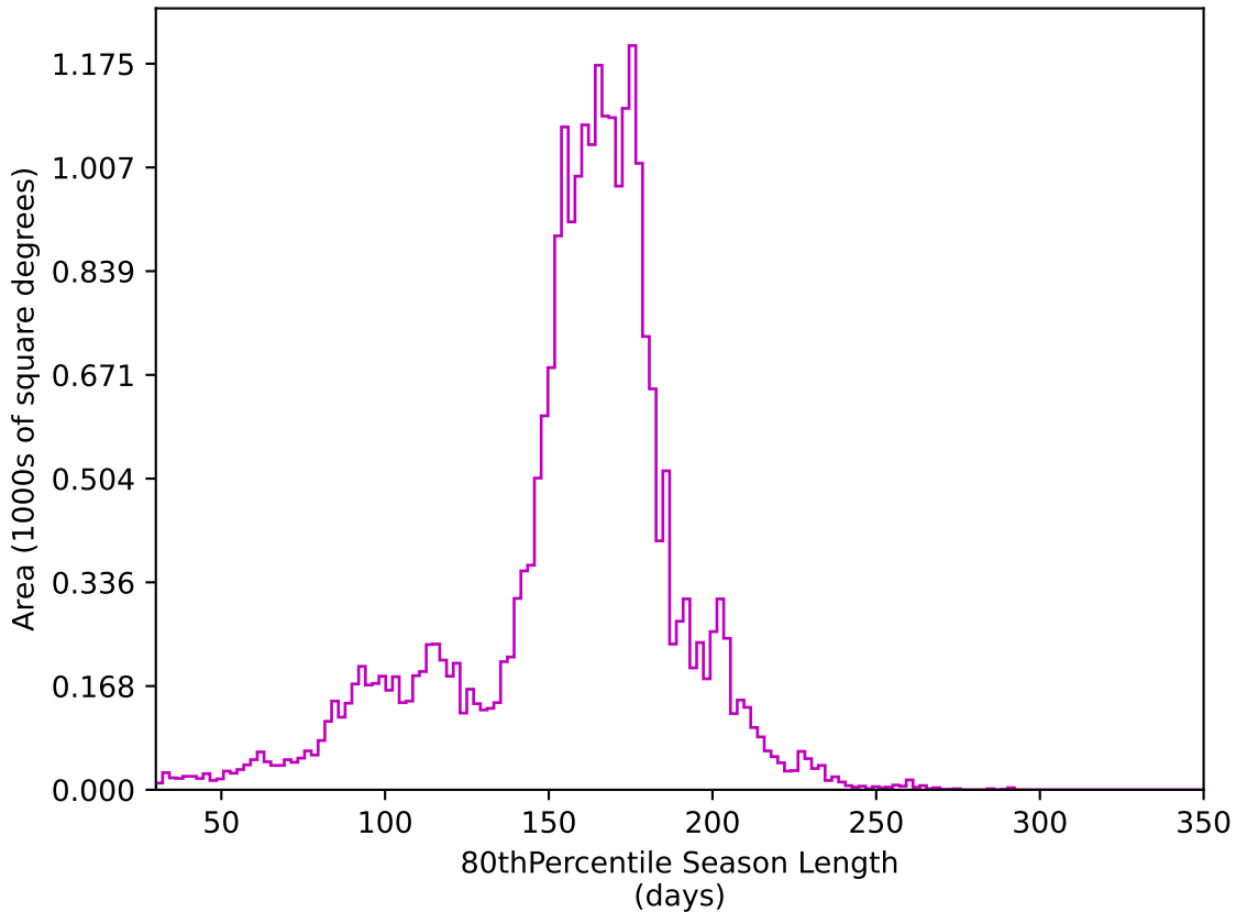
ddf_loaded_fl8_v3.4_10yrs All sky z band: 80thPercentile Season Length
