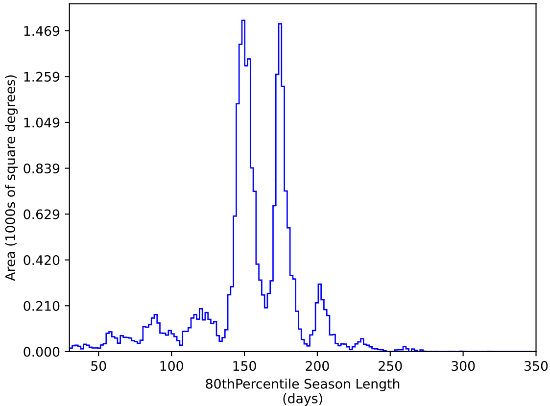
ddf_loaded_fl8_v3.4_10yrs All sky y band: 80thPercentile Season Length
