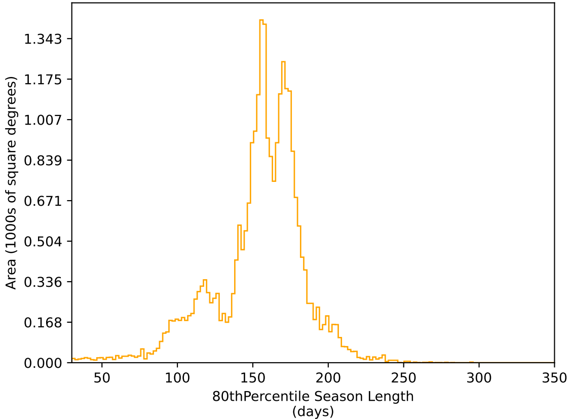
ddf_loaded_fl8_v3.4_10yrs All sky r band: 80thPercentile Season Length
