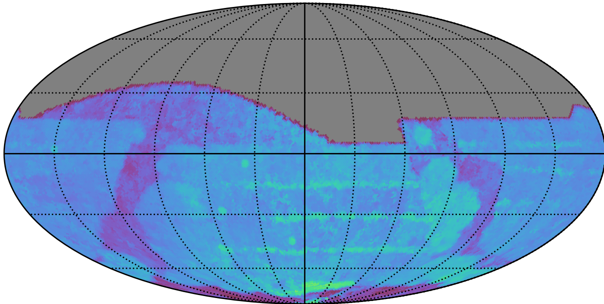
ddf_loaded_fl8_v3.4_10yrs All sky i band: 80thPercentile Season Length
