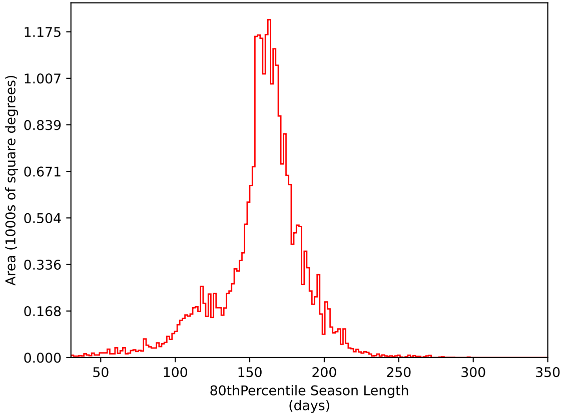
ddf_loaded_fl8_v3.4_10yrs All sky i band: 80thPercentile Season Length
