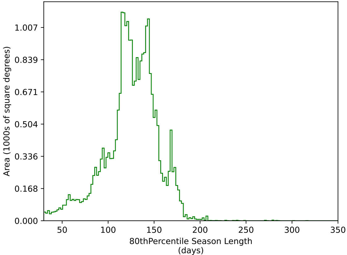
ddf_loaded_fl8_v3.4_10yrs All sky g band: 80thPercentile Season Length
