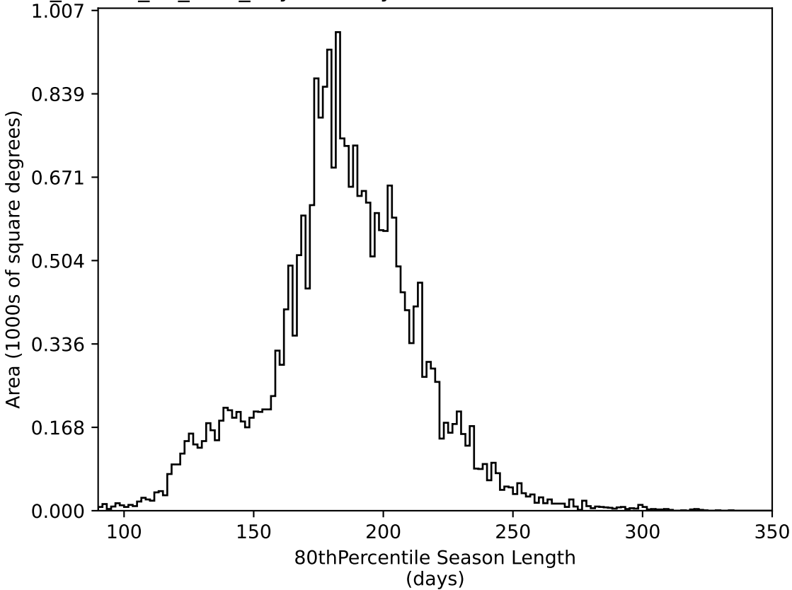
ddf_loaded_fl8_v3.4_10yrs All sky all bands: 80thPercentile Season Length
