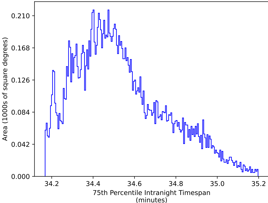
ddf_loaded_fl8_v3.4_10yrs WFD zy bands: 75th Percentile Intranight Timespan
