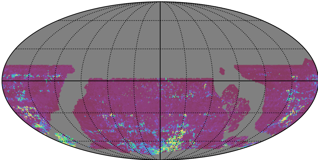
ddf_loaded_fl8_v3.4_10yrs WFD z band: 75th Percentile Intranight Timespan
