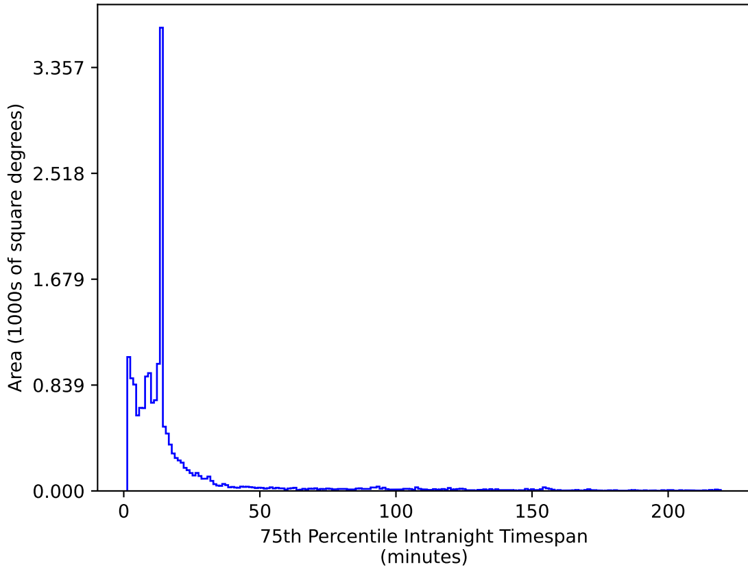
ddf_loaded_fl8_v3.4_10yrs WFD z band: 75th Percentile Intranight Timespan
