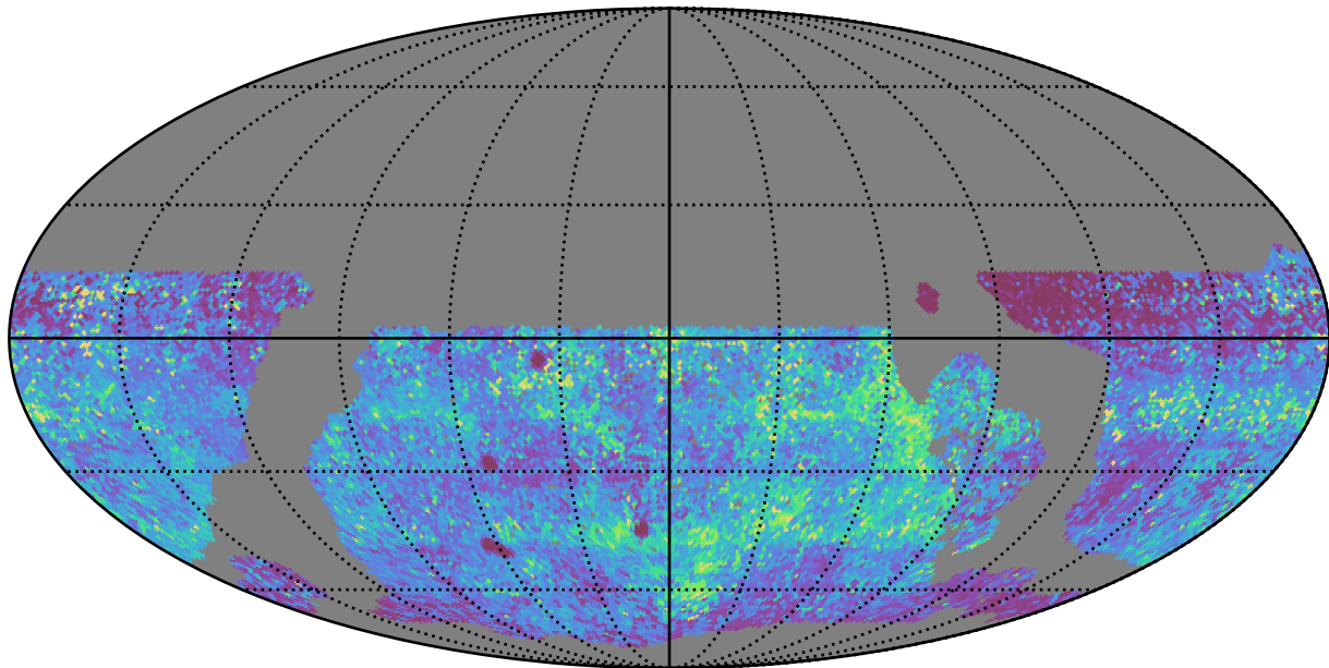
ddf_loaded_fl8_v3.4_10yrs WFD y band: 75th Percentile Intranight Timespan
