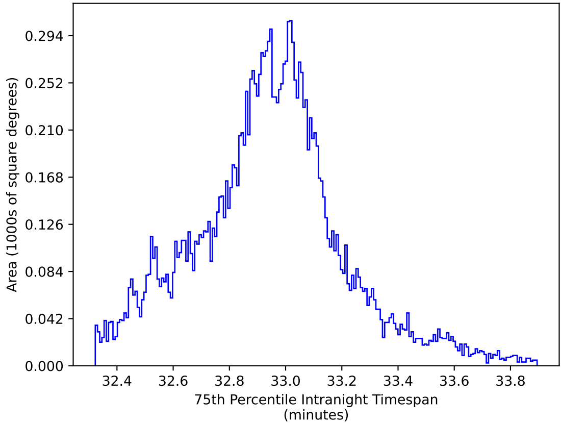
ddf_loaded_fl8_v3.4_10yrs WFD y band: 75th Percentile Intranight Timespan
