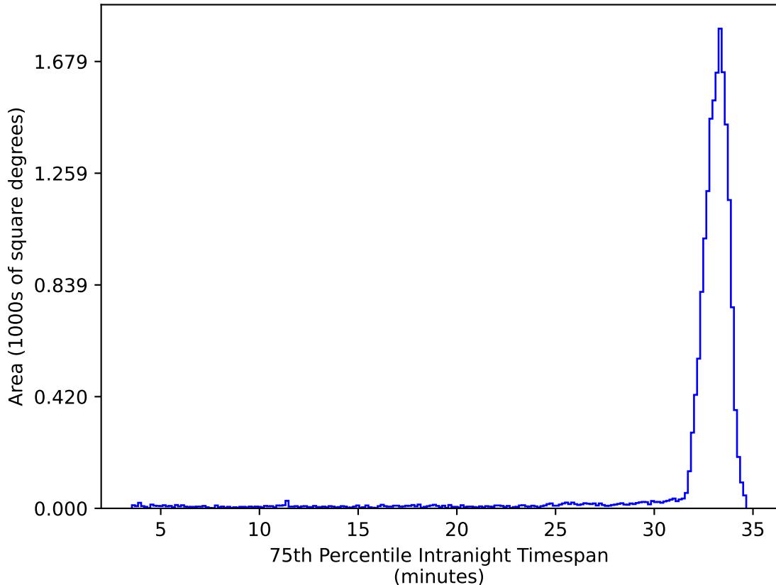
ddf_loaded_fl8_v3.4_10yrs WFD ug bands: 75th Percentile Intranight Timespan
