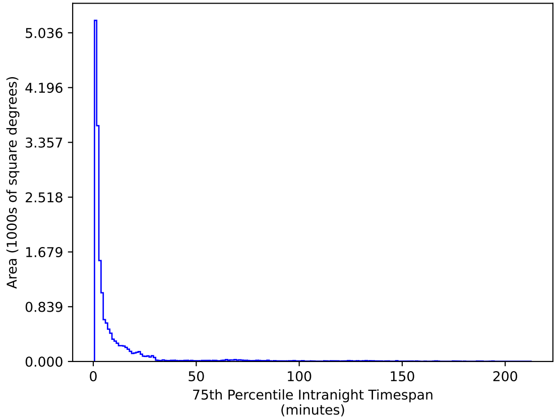
ddf_loaded_fl8_v3.4_10yrs WFD u band: 75th Percentile Intranight Timespan
