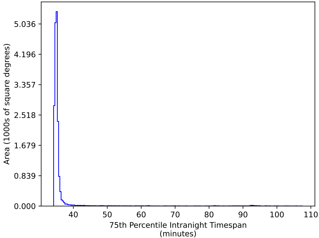
ddf_loaded_fl8_v3.4_10yrs WFD ri bands: 75th Percentile Intranight Timespan
