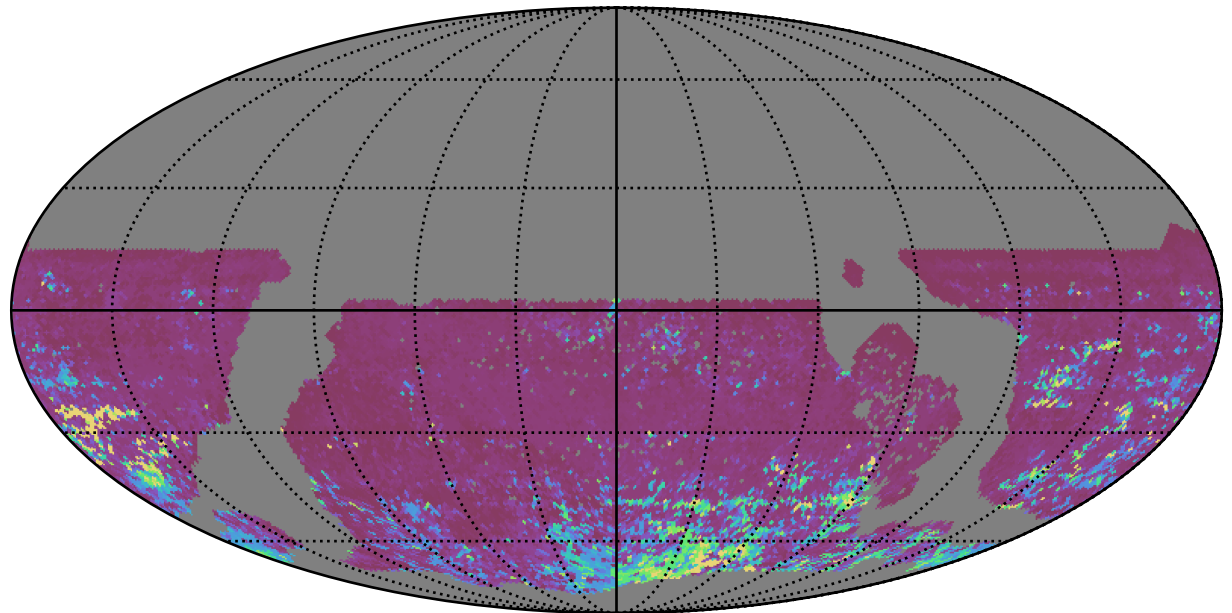
ddf_loaded_fl8_v3.4_10yrs WFD i band: 75th Percentile Intranight Timespan
