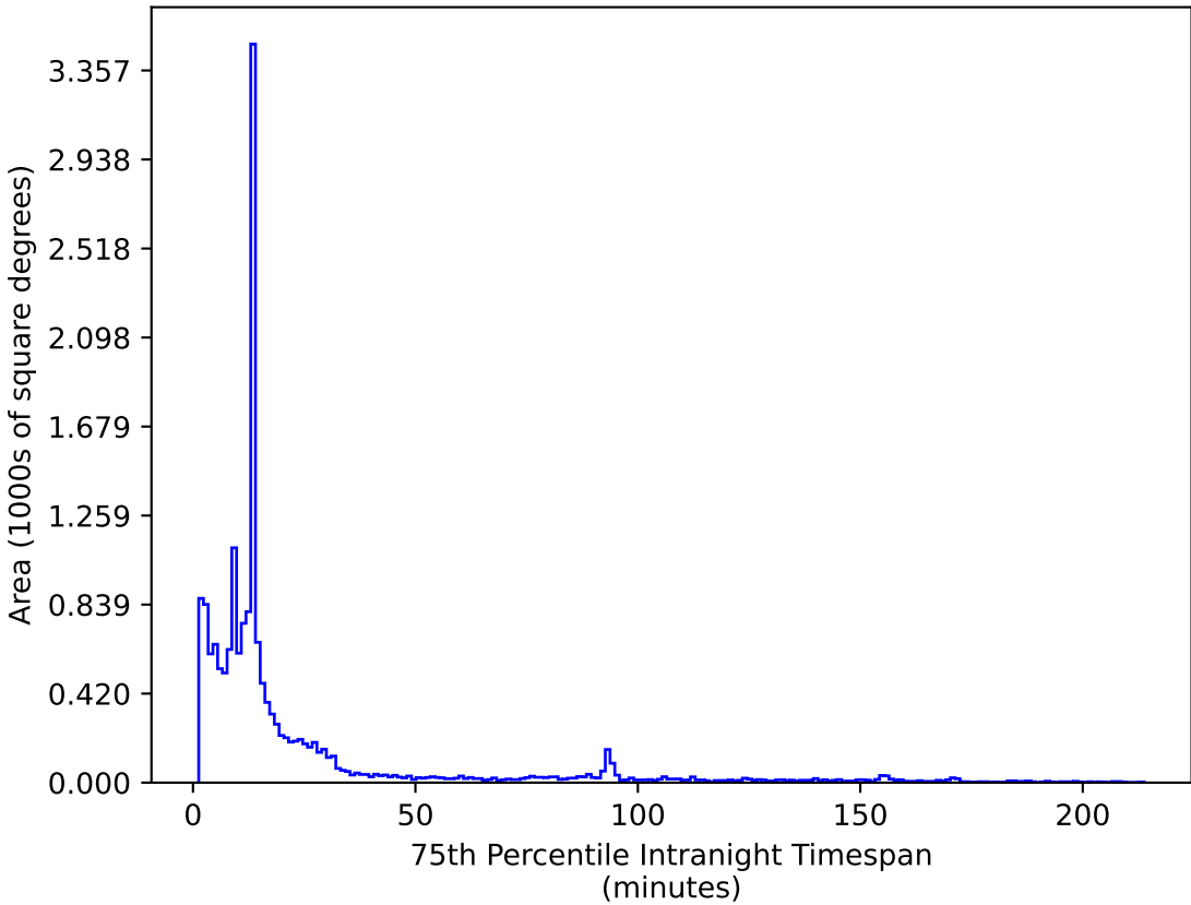
ddf_loaded_fl8_v3.4_10yrs WFD i band: 75th Percentile Intranight Timespan
