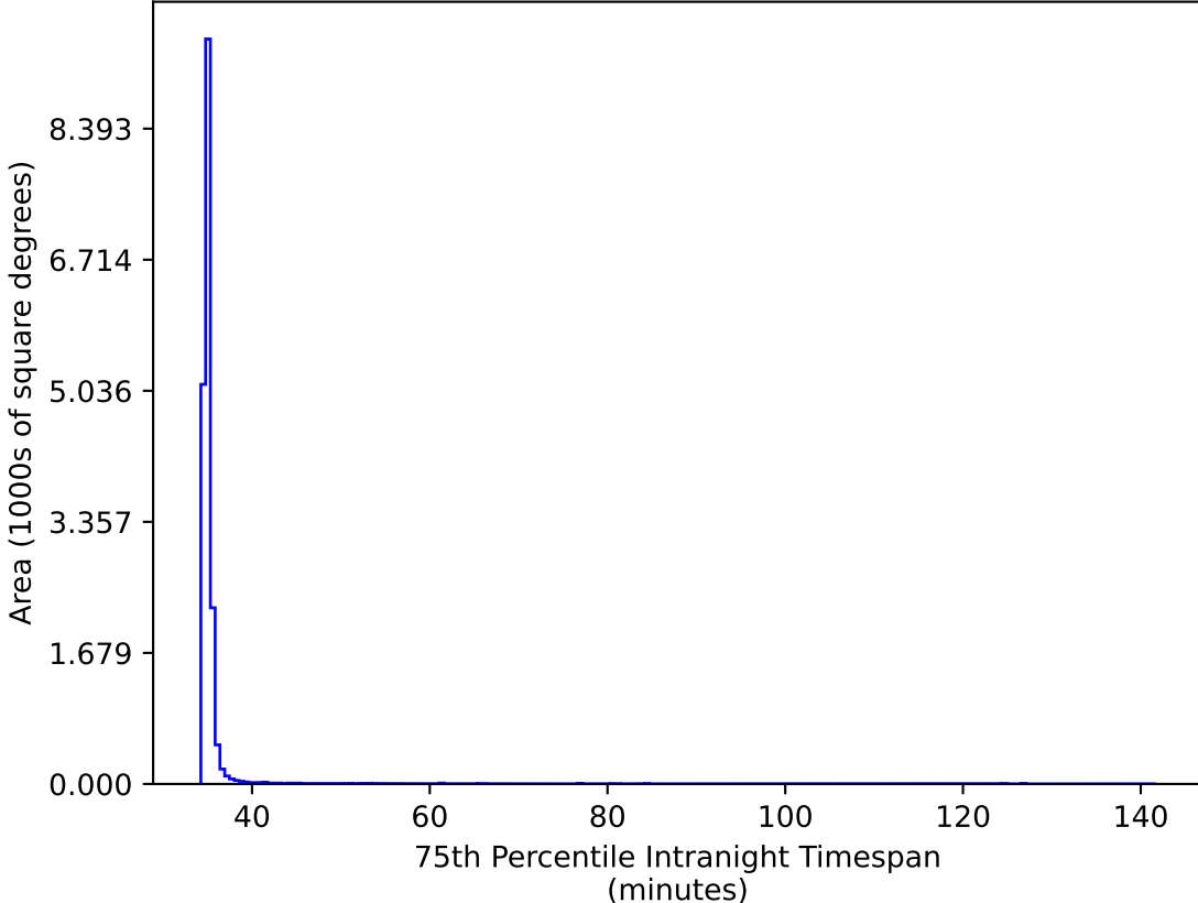
ddf_loaded_fl8_v3.4_10yrs WFD gr bands: 75th Percentile Intranight Timespan
