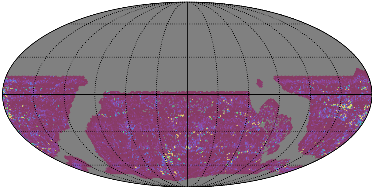
ddf_loaded_fl8_v3.4_10yrs WFD g band: 75th Percentile Intranight Timespan
