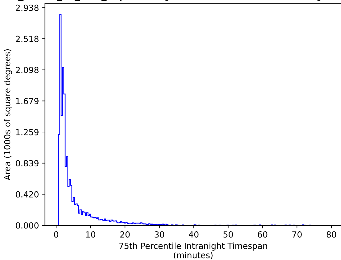
ddf_loaded_fl8_v3.4_10yrs WFD g band: 75th Percentile Intranight Timespan
