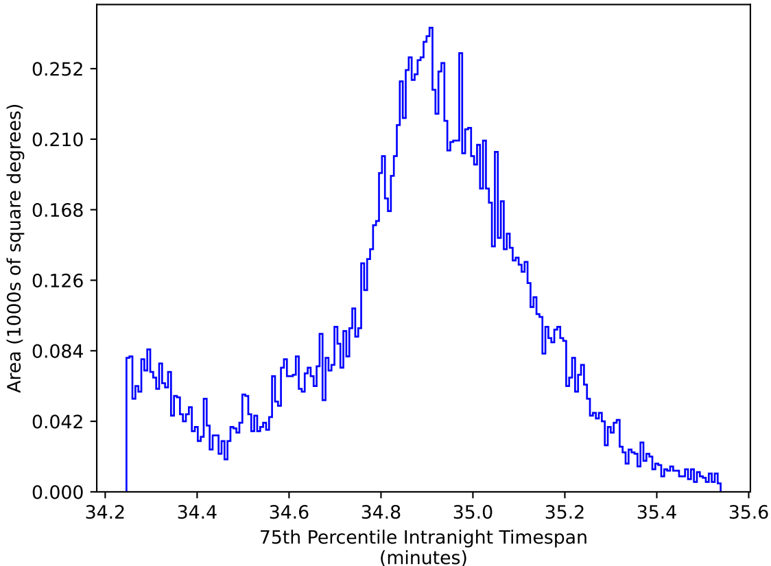
ddf_loaded_fl8_v3.4_10yrs WFD all bands: 75th Percentile Intranight Timespan
