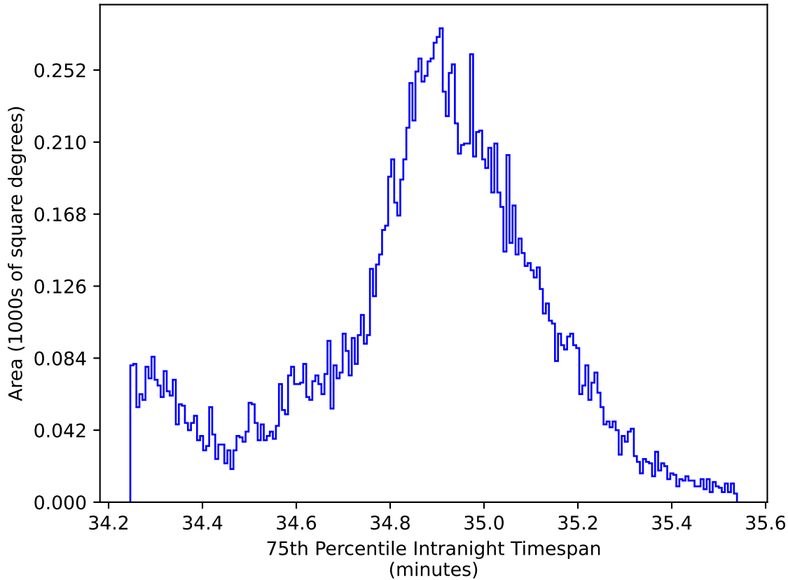
ddf_loaded_fl8_v3.4_10yrs WFD: 75th Percentile Intranight Timespan
