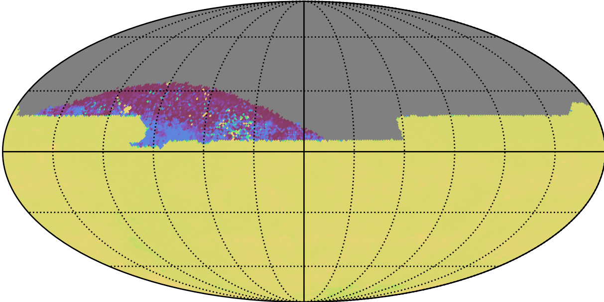
ddf_loaded_fl8_v3.4_10yrs All sky zy bands: 75th Percentile Intranight Timespan
