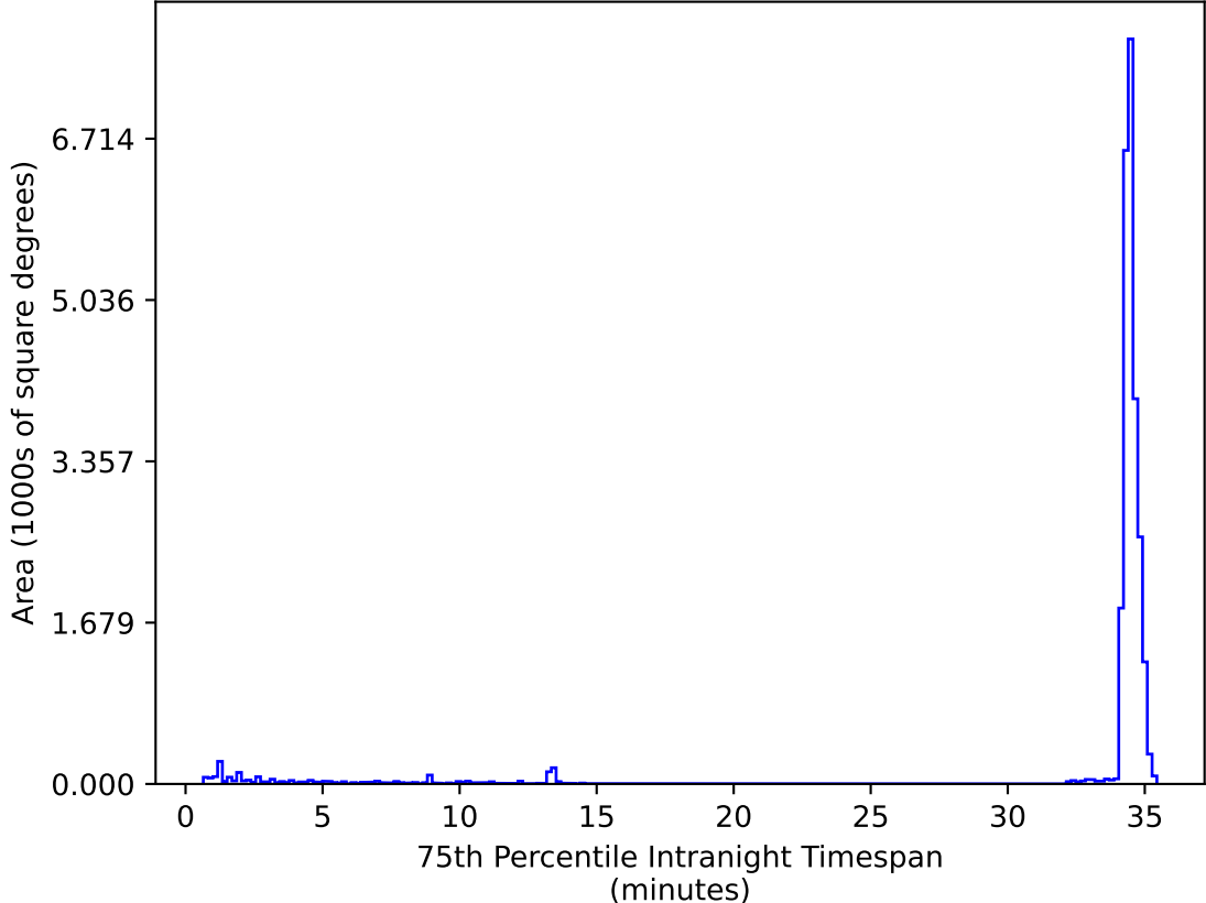
ddf_loaded_fl8_v3.4_10yrs All sky zy bands: 75th Percentile Intranight Timespan
