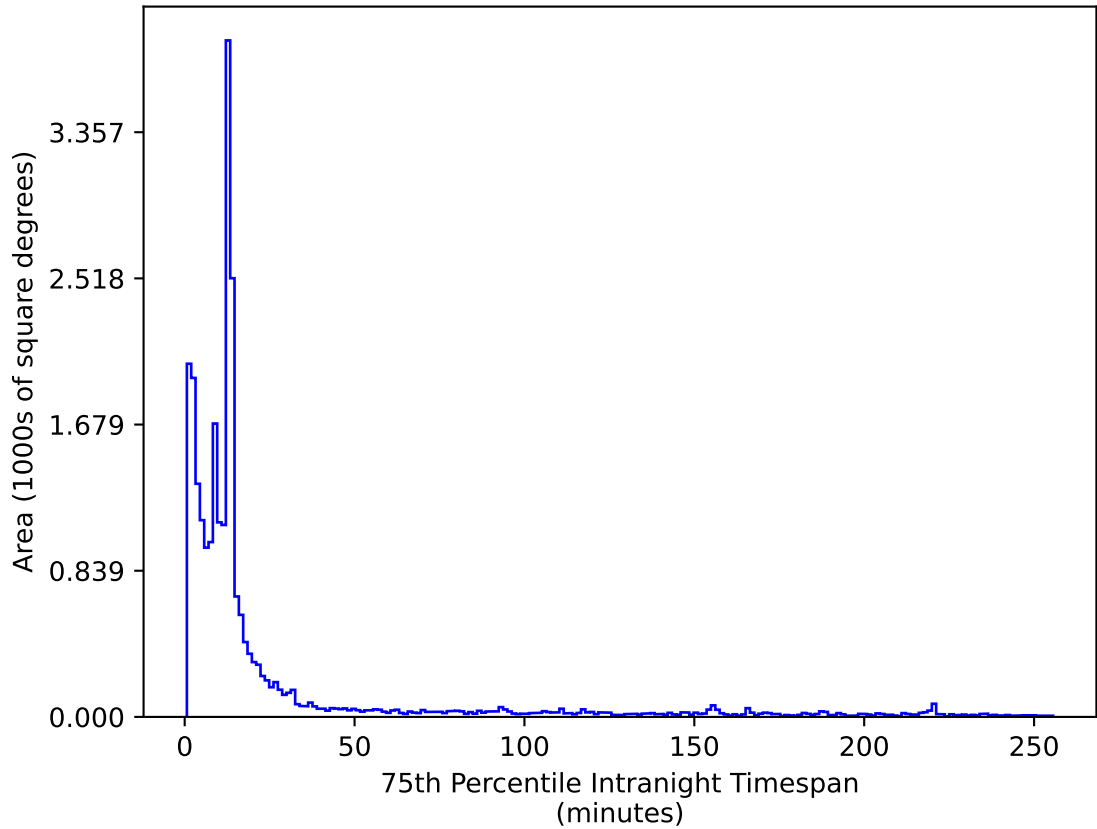
ddf_loaded_fl8_v3.4_10yrs All sky z band: 75th Percentile Intranight Timespan
