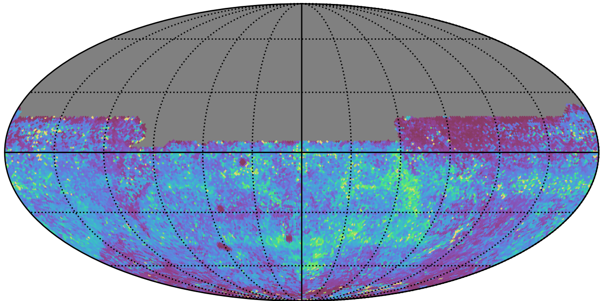
ddf_loaded_fl8_v3.4_10yrs All sky y band: 75th Percentile Intranight Timespan
