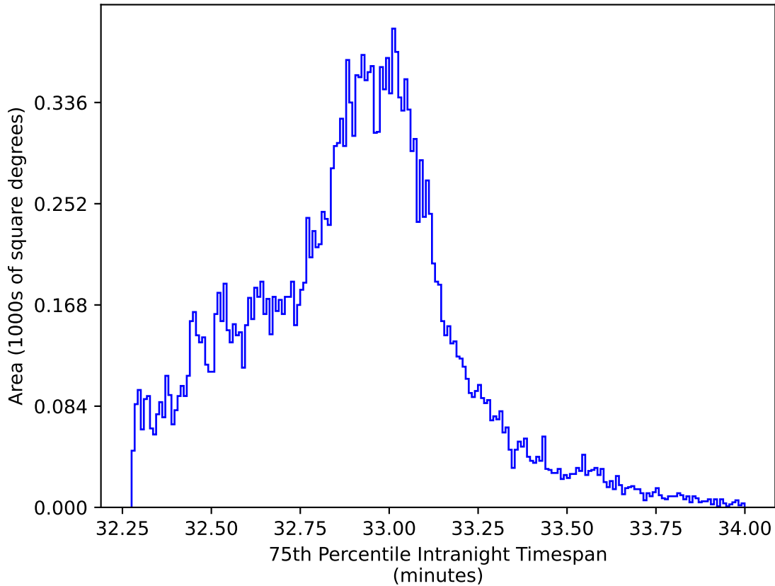
ddf_loaded_fl8_v3.4_10yrs All sky y band: 75th Percentile Intranight Timespan
