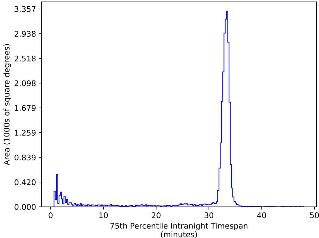
ddf_loaded_fl8_v3.4_10yrs All sky ug bands: 75th Percentile Intranight Timespan
