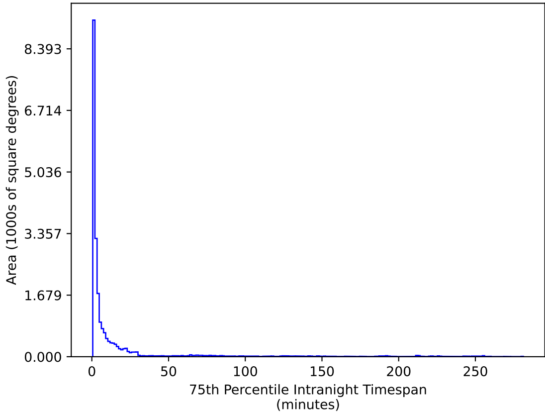
ddf_loaded_fl8_v3.4_10yrs All sky u band: 75th Percentile Intranight Timespan
