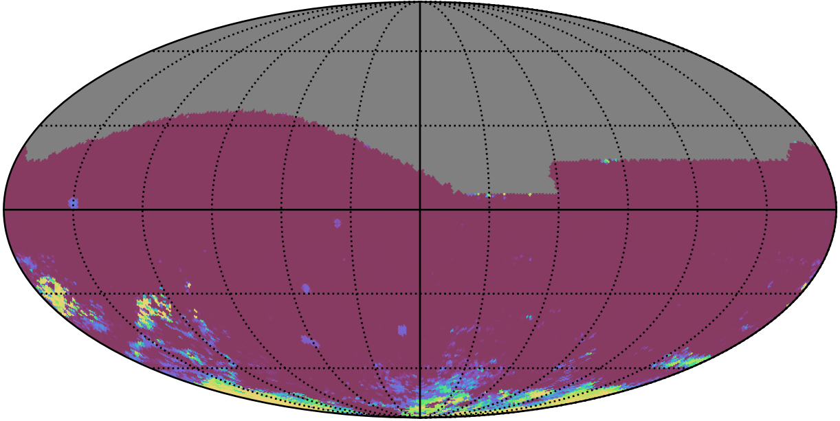
ddf_loaded_fl8_v3.4_10yrs All sky ri bands: 75th Percentile Intranight Timespan
