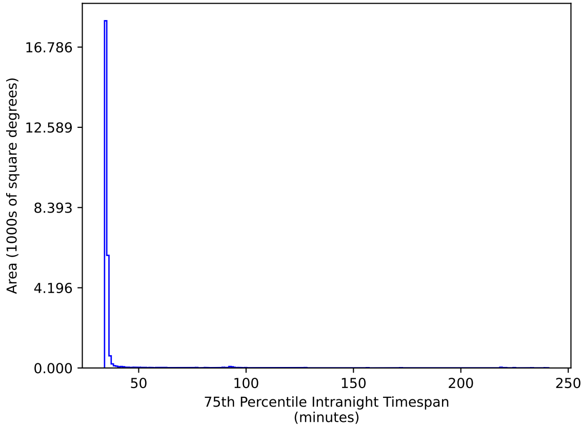
ddf_loaded_fl8_v3.4_10yrs All sky ri bands: 75th Percentile Intranight Timespan
