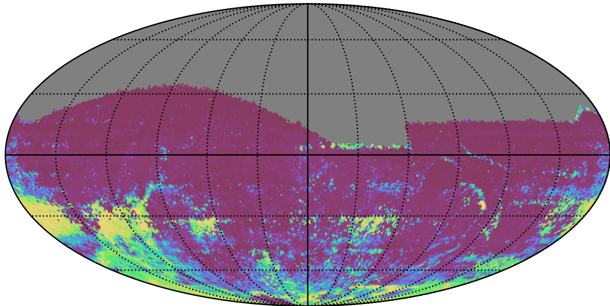
ddf_loaded_fl8_v3.4_10yrs All sky r band: 75th Percentile Intranight Timespan
