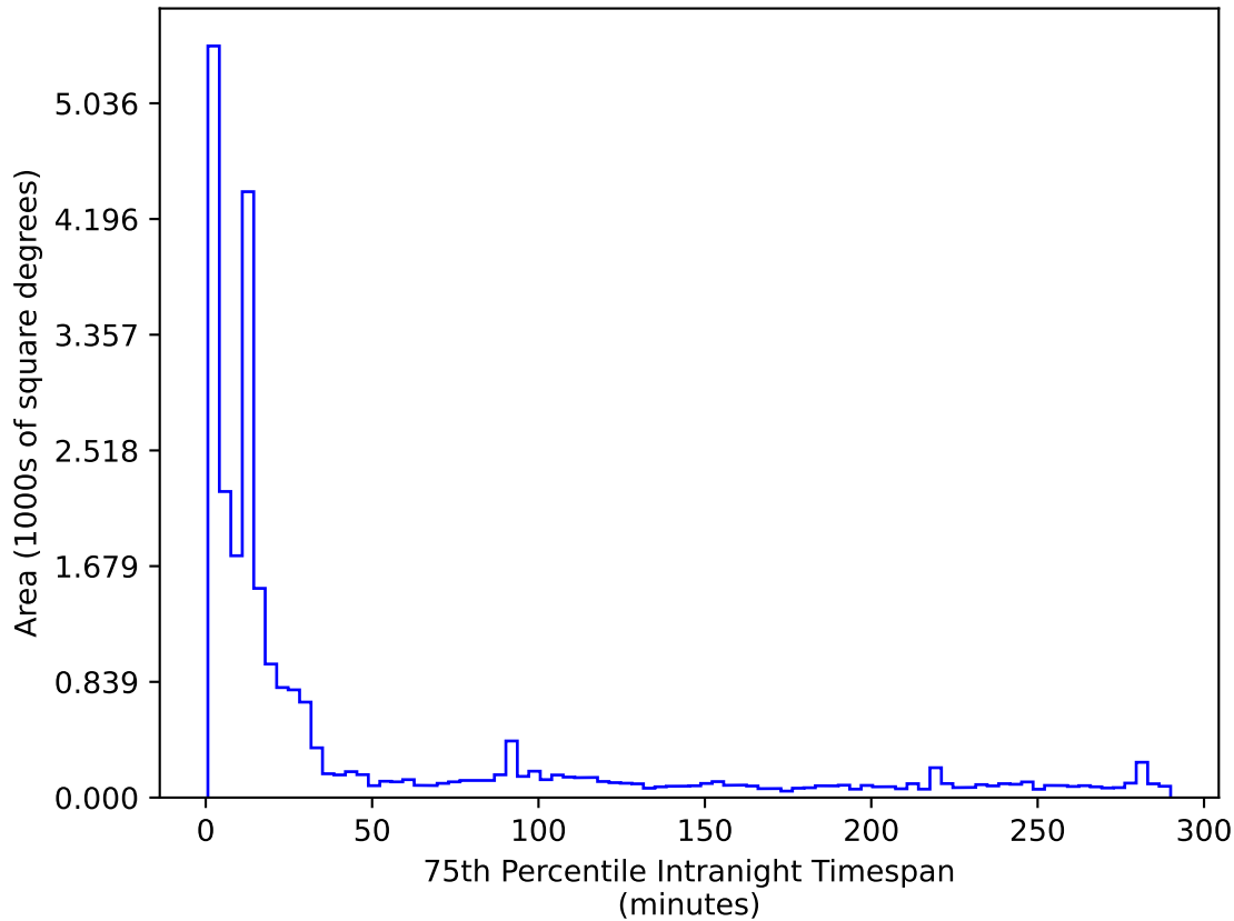
ddf_loaded_fl8_v3.4_10yrs All sky r band: 75th Percentile Intranight Timespan
