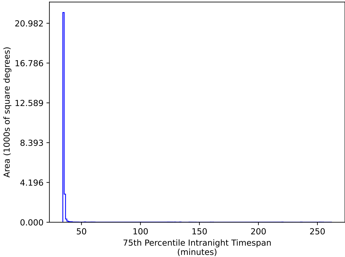
ddf_loaded_fl8_v3.4_10yrs All sky gr bands: 75th Percentile Intranight Timespan
