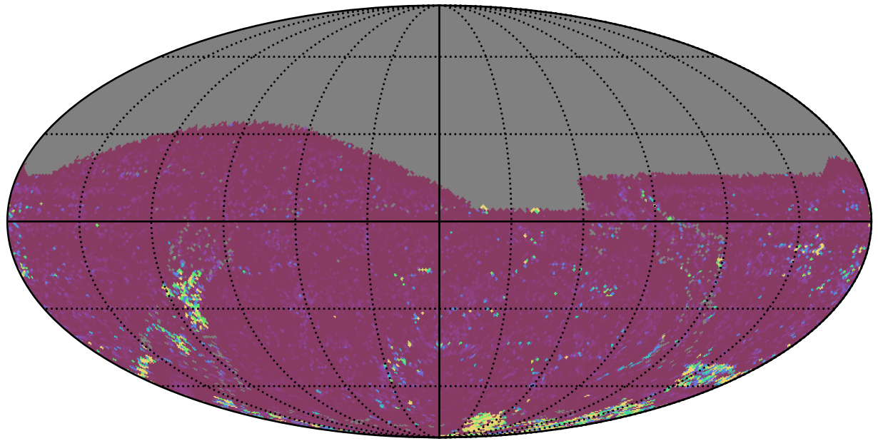
ddf_loaded_fl8_v3.4_10yrs All sky g band: 75th Percentile Intranight Timespan
